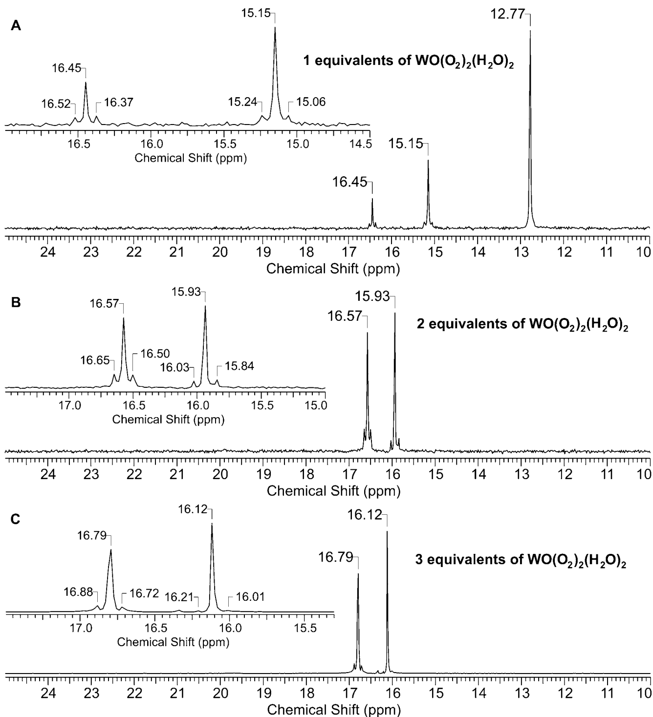
Figure 1. ^{31}\text{P} NMR spectra of 4\text{-MePhPO(ONa)}_2 in a \text{H}_2\text{O}/\text{H}_2\text{O}_2/\text{CD}_3\text{CN} mixture in the presence of different amounts of [\text{W(O)(O}_2)_2(\text{H}_2\text{O})_2] .
